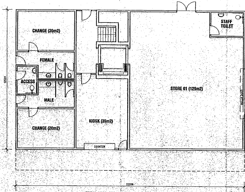
1. GROUND FLOOR PLAN 1:100
