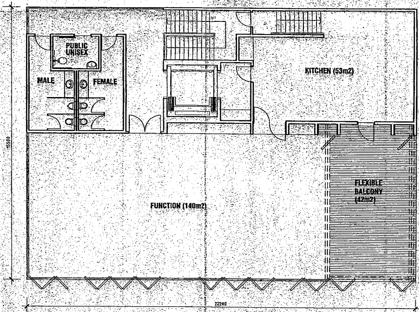
1. LEVEL 1 FLOOR PLAN 1:100
